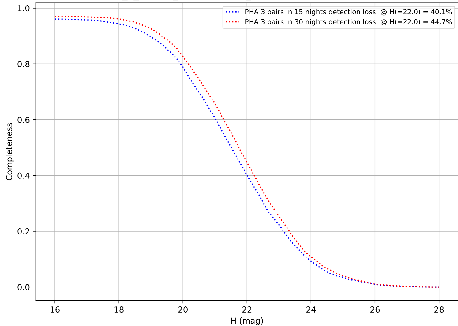
internal_u_expt30_nscale0.9v3.4_10yrs: DifferentialCompleteness
