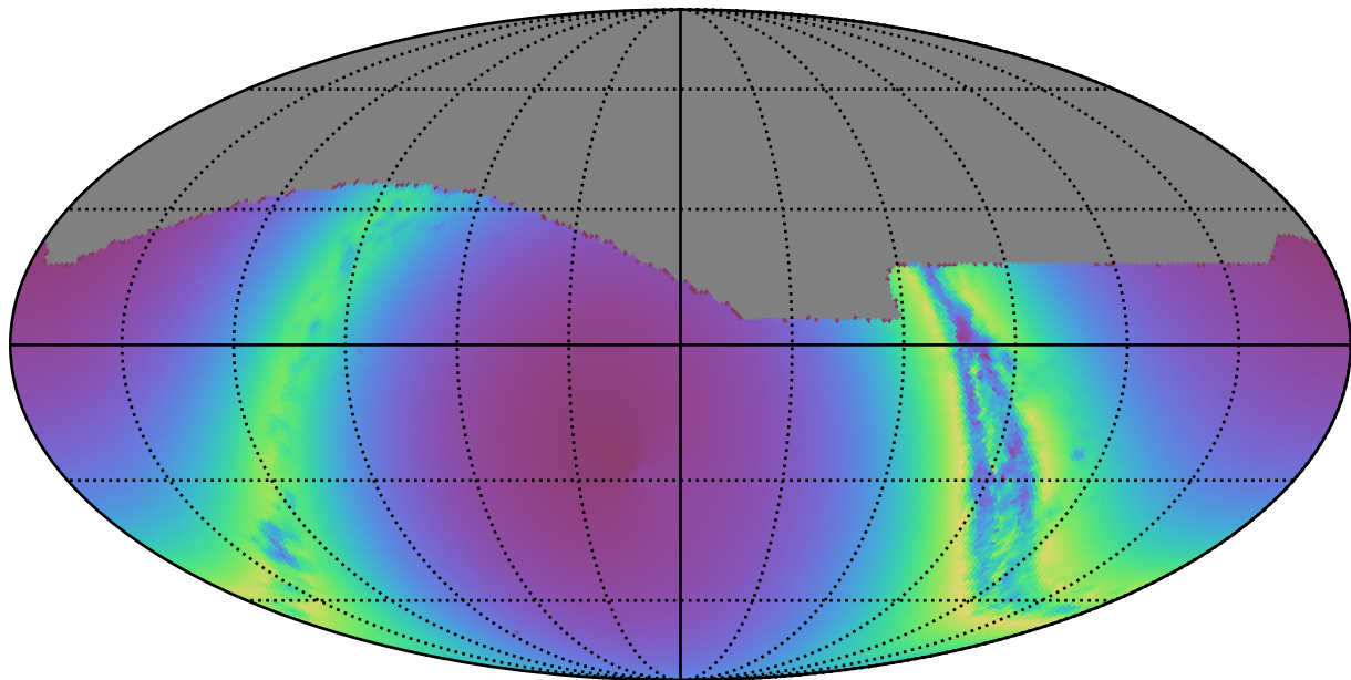
internal_u_expt30_nscale0.9v3.4_10yrs : young_stars
