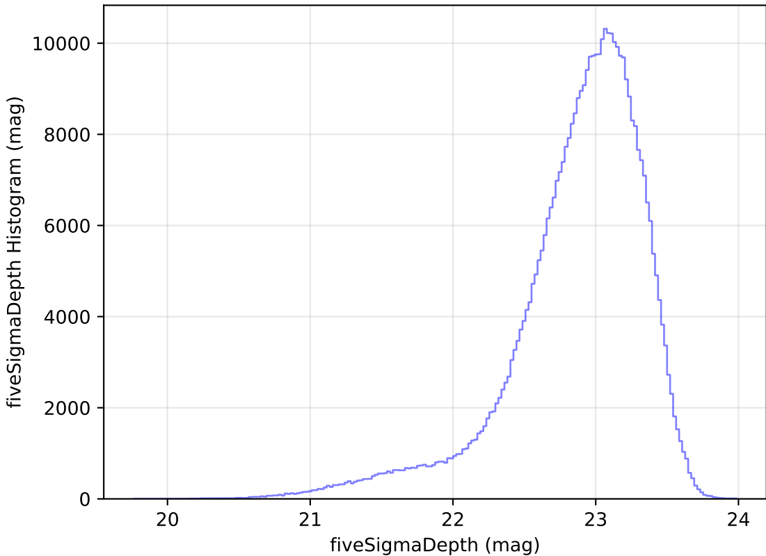
internal_u_expt30_nscale0.9v3.4_10yrs z: fiveSigmaDepth Histogram
