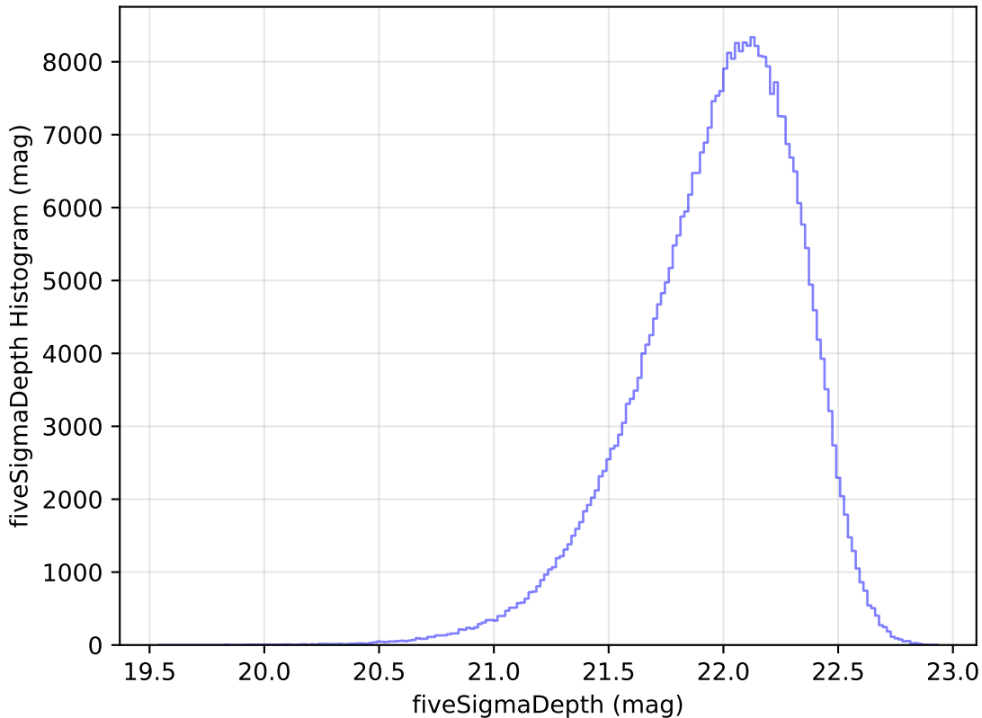
internal_u_expt30_nscale0.9v3.4_10yrs y: fiveSigmaDepth Histogram
