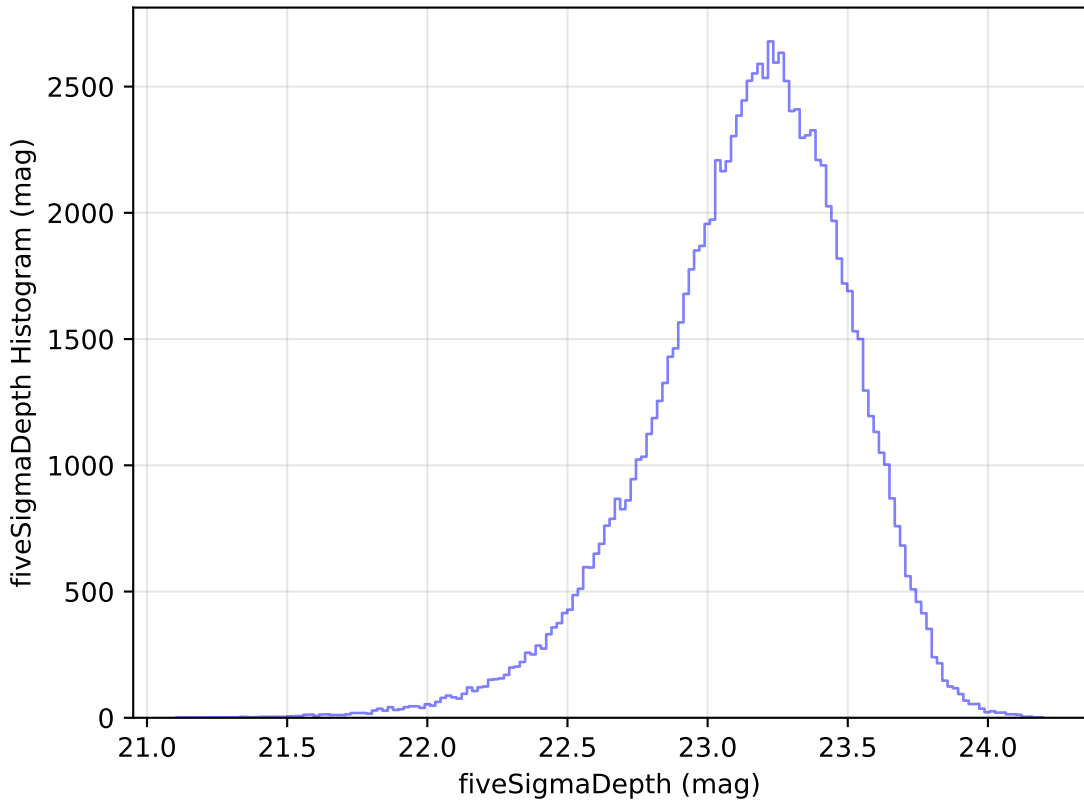
internal_u_expt30_nscale0.9v3.4_10yrs u: fiveSigmaDepth Histogram
