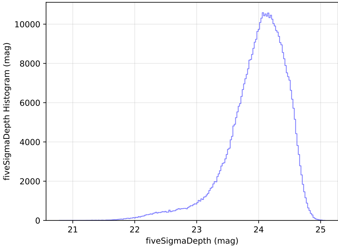
internal_u_expt30_nscale0.9v3.4_10yrs r: fiveSigmaDepth Histogram
