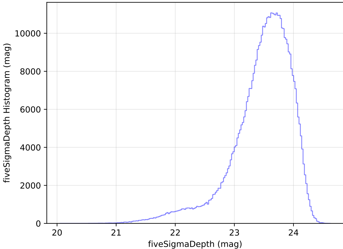
internal_u_expt30_nscale0.9v3.4_10yrs i: fiveSigmaDepth Histogram
