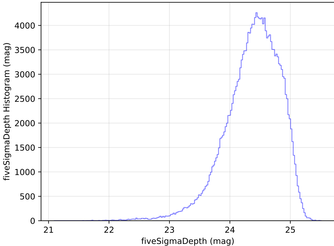
internal_u_expt30_nscale0.9v3.4_10yrs g: fiveSigmaDepth Histogram
