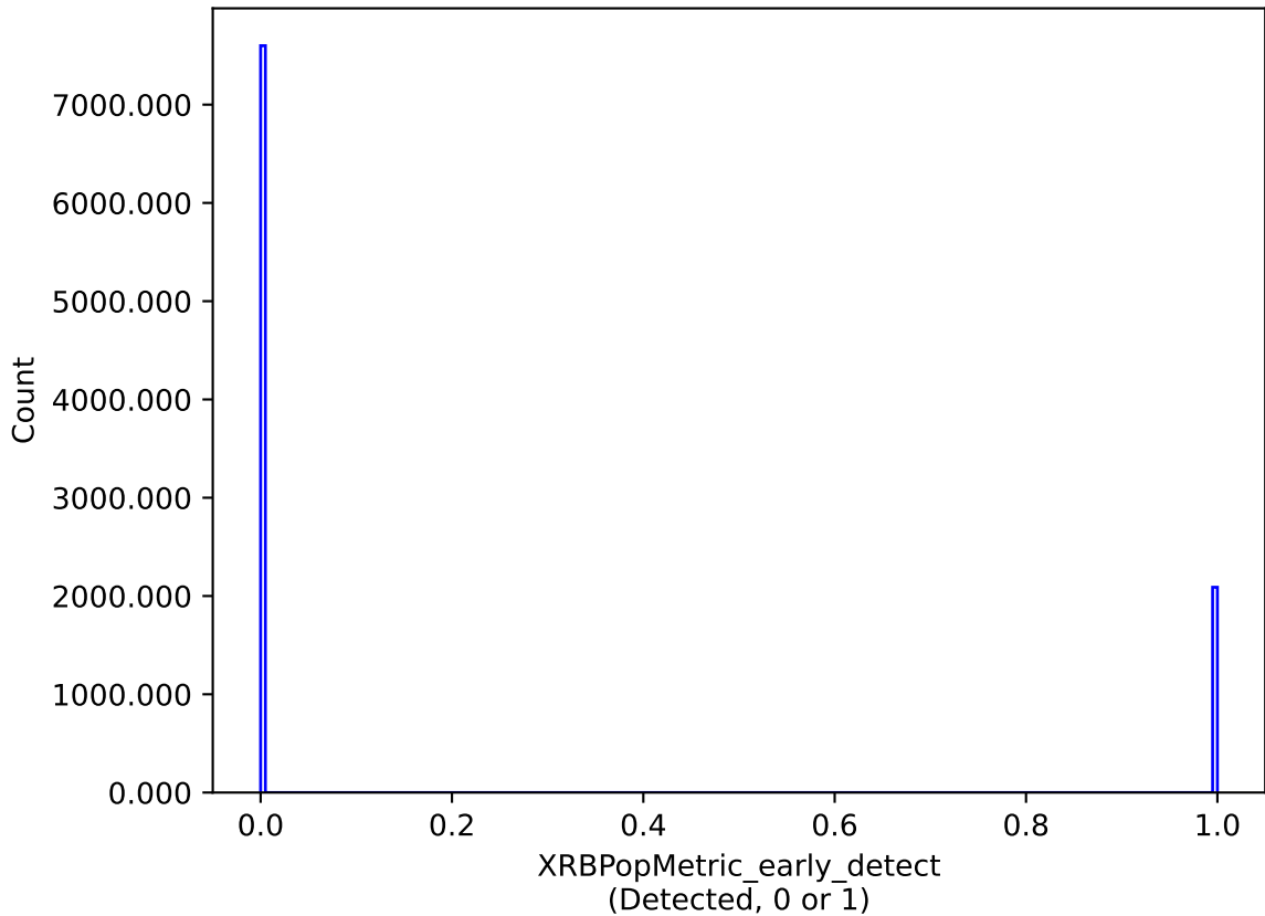
internal_u_expt30_nscale0.9v3.4_10yrs : XRBPoMetric_early_detect
