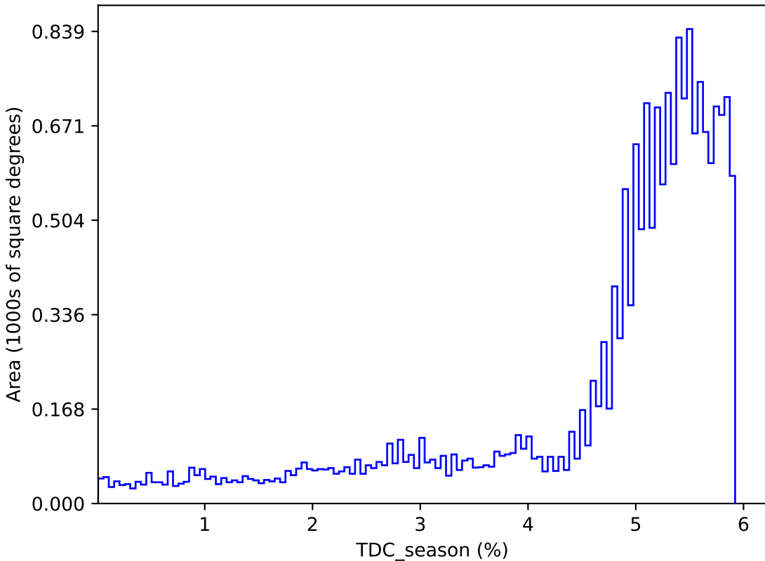
internal_u_expt30_nscale0.9v3.4_10yrs : TDC_season
