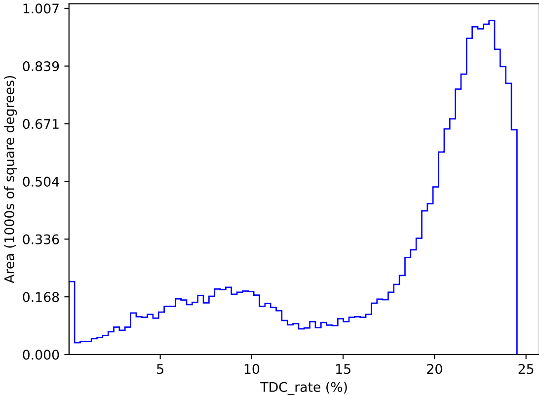
internal_u_expt30_nscale0.9v3.4_10yrs : TDC_rate
