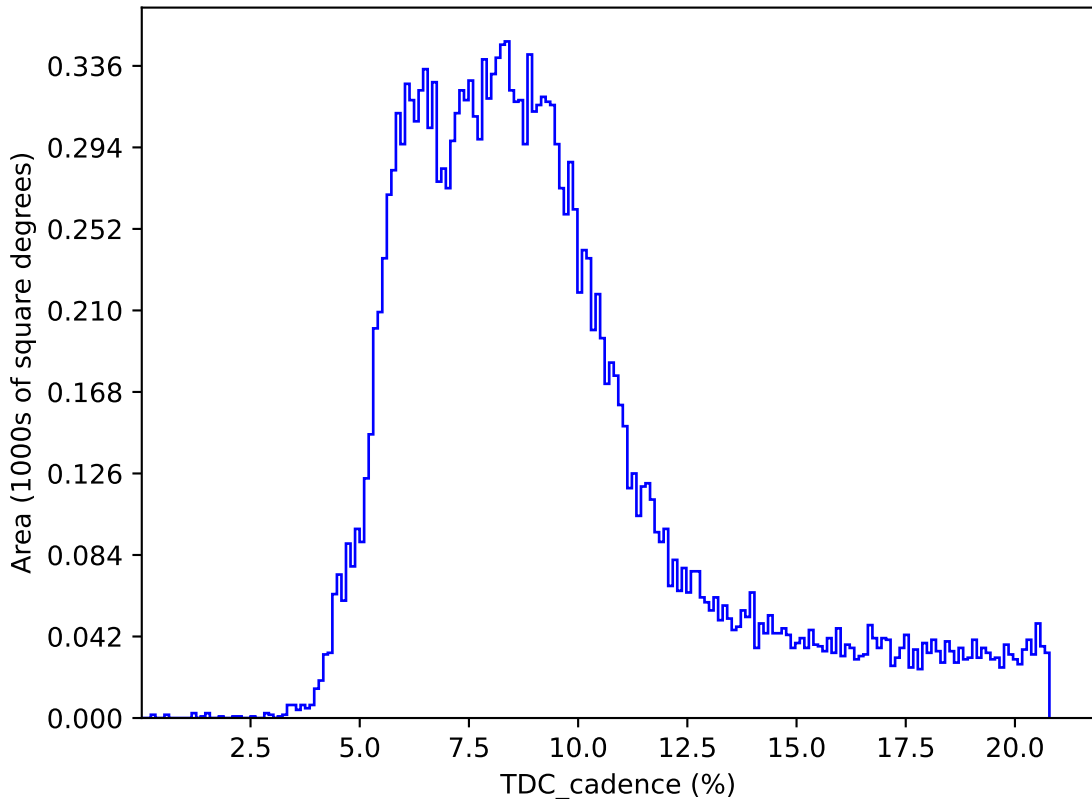
internal_u_expt30_nscale0.9v3.4_10yrs : TDC_cadence
