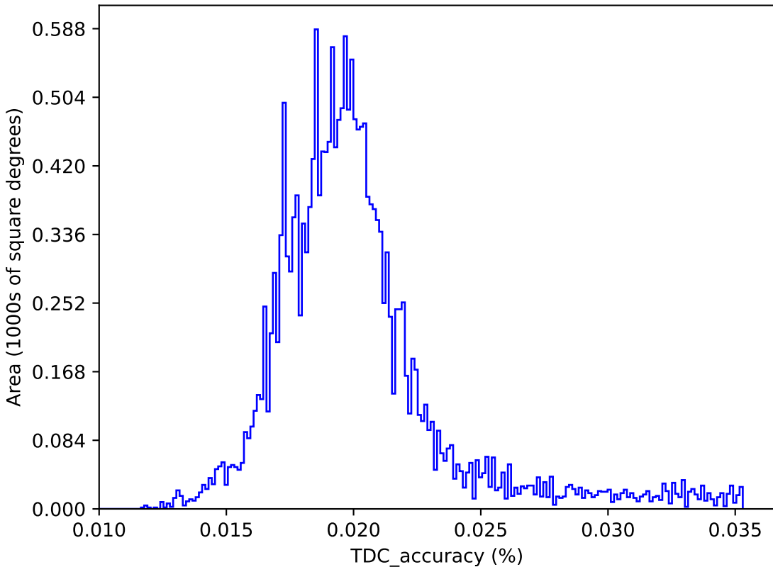
internal_u_expt30_nscale0.9v3.4_10yrs : TDC_accuracy
