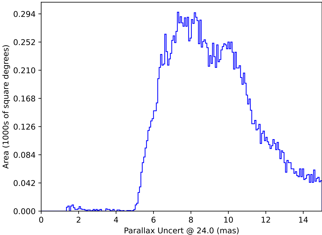
internal_u_expt30_nscale0.9v3.4_10yrs : Parallax Uncert @ 24.0
