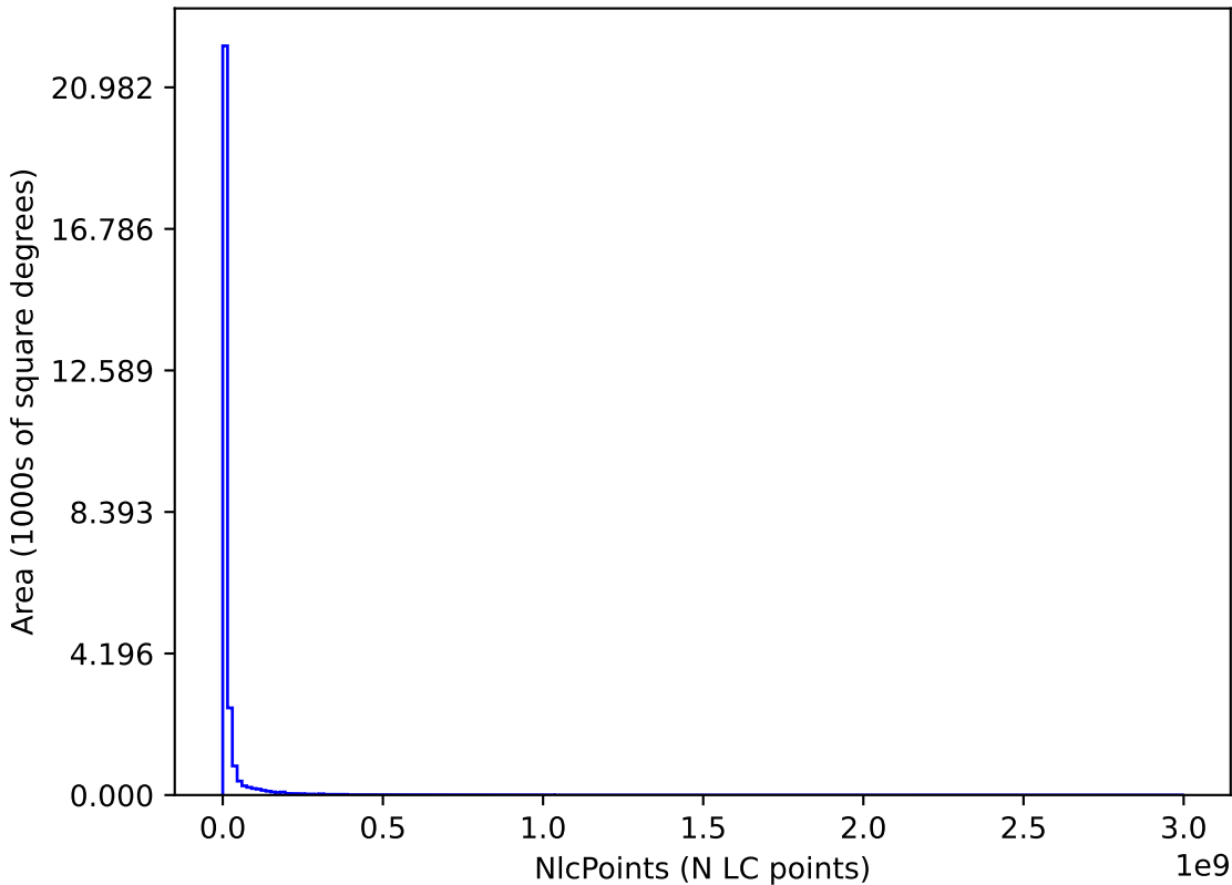
internal_u_expt30_nscale0.9v3.4_10yrs : NlcPoints
