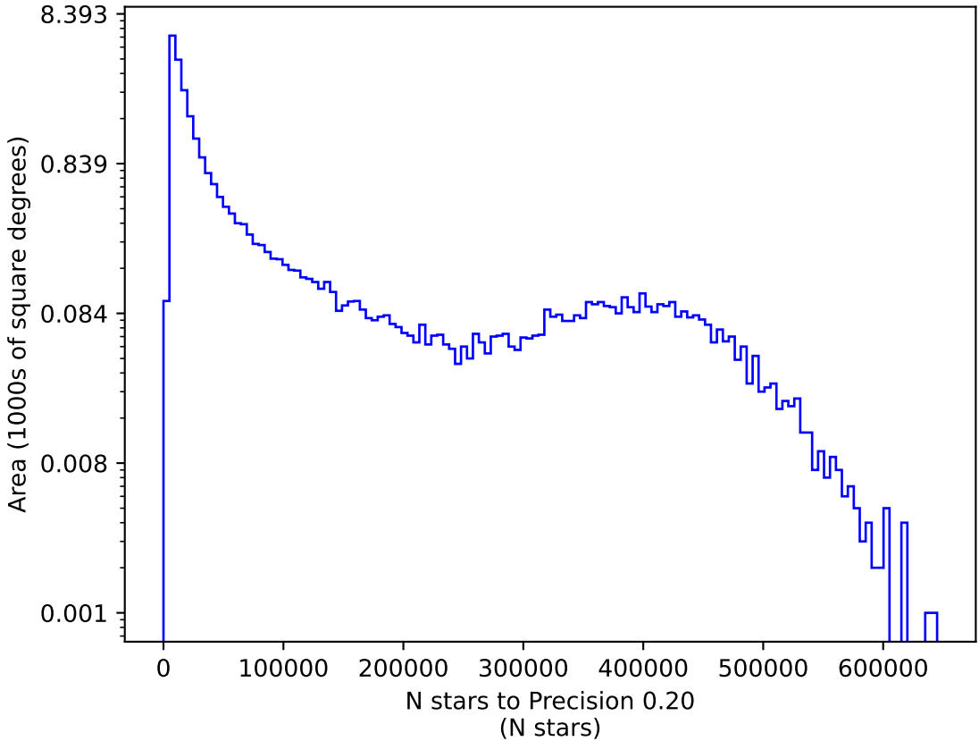
internal_u_expt30_nscale0.9v3.4_10yrs z: N stars to Precision 0.20
