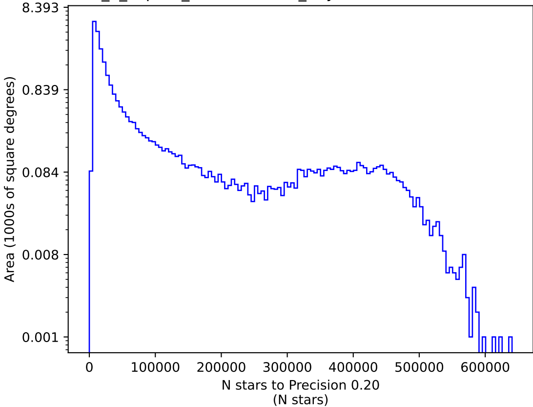
internal_u_expt30_nscale0.9v3.4_10yrs i: N stars to Precision 0.20
