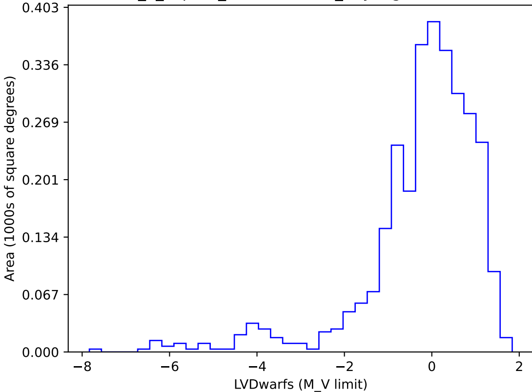
internal_u_expt30_nscale0.9v3.4_10yrs gi SCP: LVDwarfs
