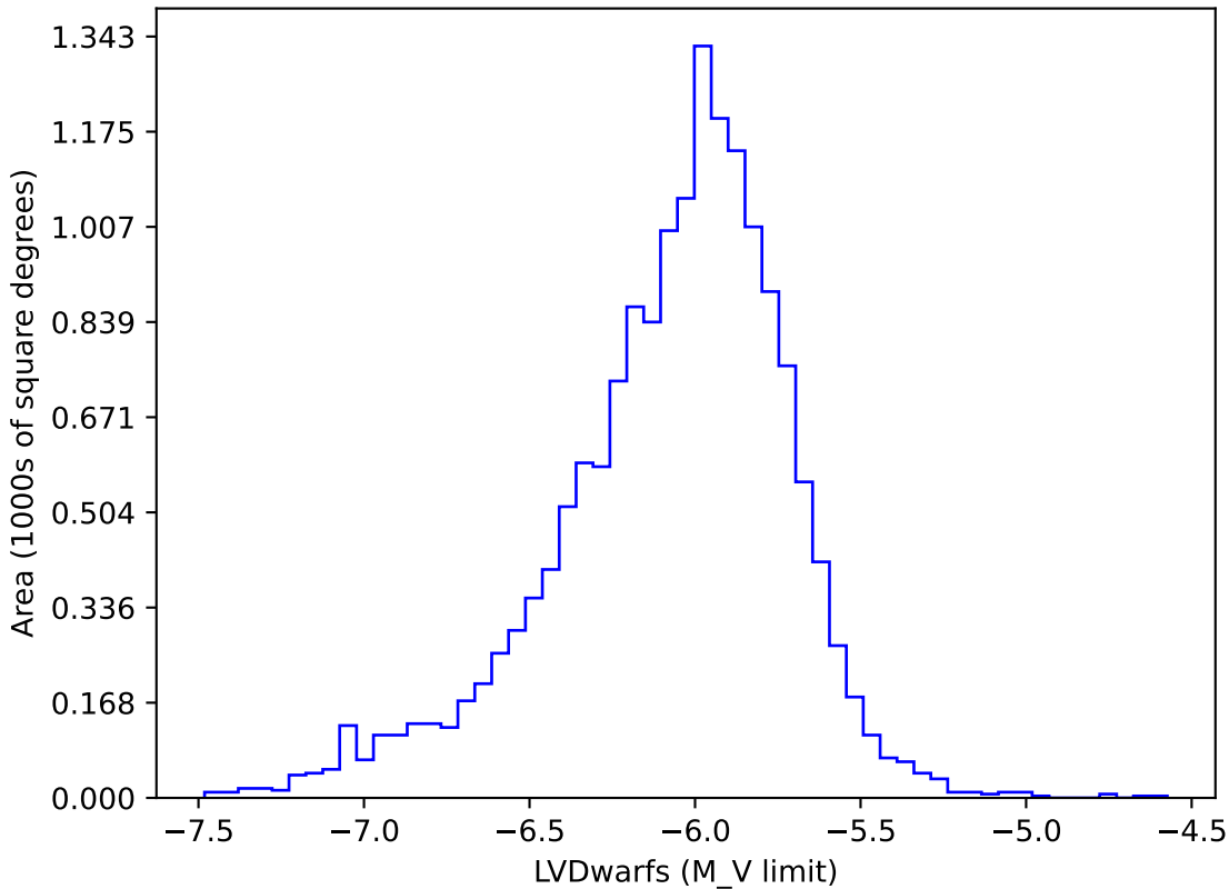
internal_u_expt30_nscale0.9v3.4_10yrs gi: LVDwarfs
