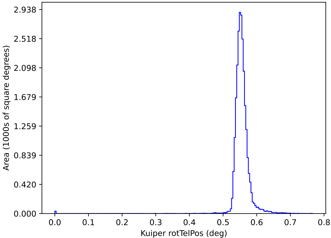
internal_u_expt30_nscale0.9v3.4_10yrs y: Kuiper rotTelPos
