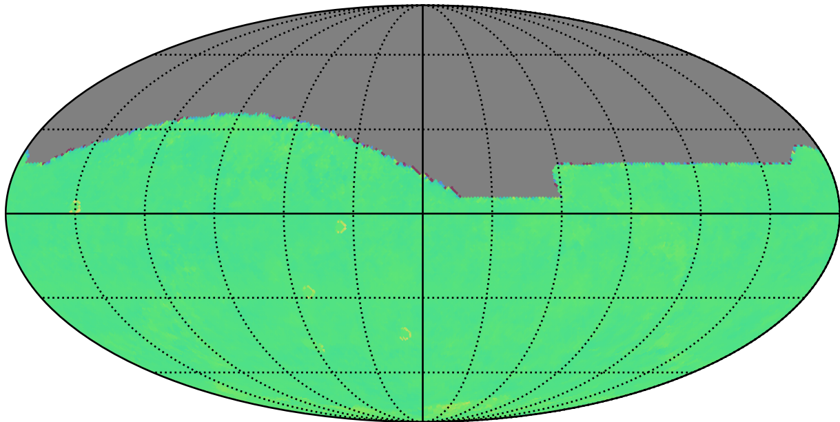
internal_u_expt30_nscale0.9v3.4_10yrs r: Kuiper rotTelPos
