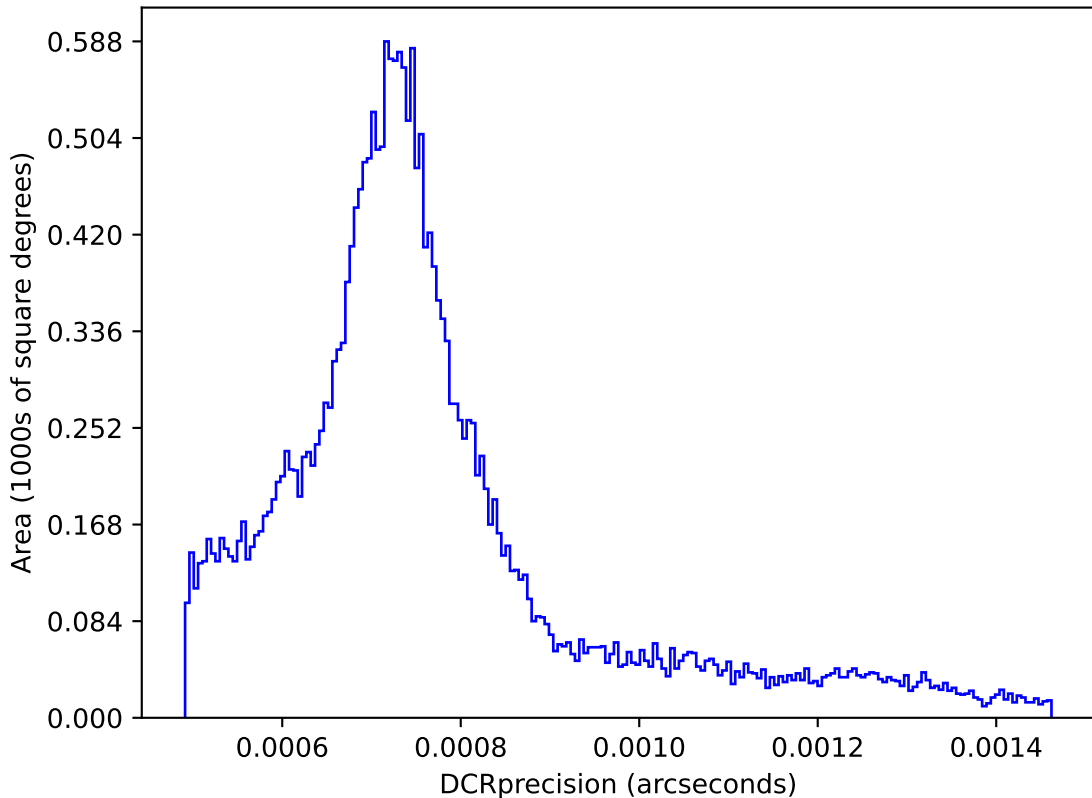
internal_u_expt30_nscale0.9v3.4_10yrs : DCRprecision
