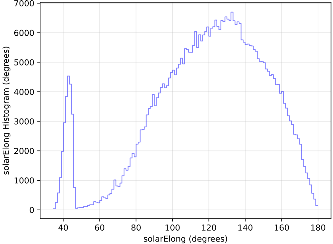
internal_u_expt30_nscale0.9v3.4_10yrs WFD z band: solarElong Histogram
