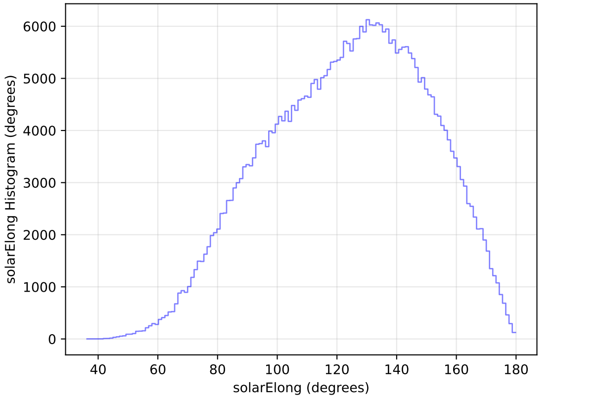
internal_u_expt30_nscale0.9v3.4_10yrs WFD y band: solarElong Histogram
