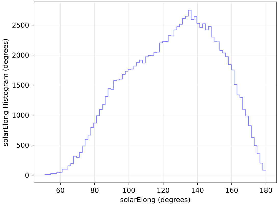
internal_u_expt30_nscale0.9v3.4_10yrs WFD u band: solarElong Histogram
