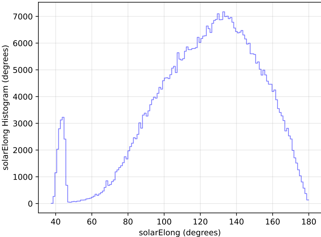
internal_u_expt30_nscale0.9v3.4_10yrs WFD r band: solarElong Histogram
