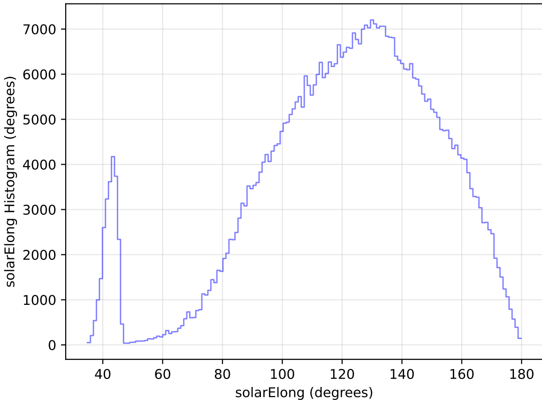
internal_u_expt30_nscale0.9v3.4_10yrs WFD i band: solarElong Histogram
