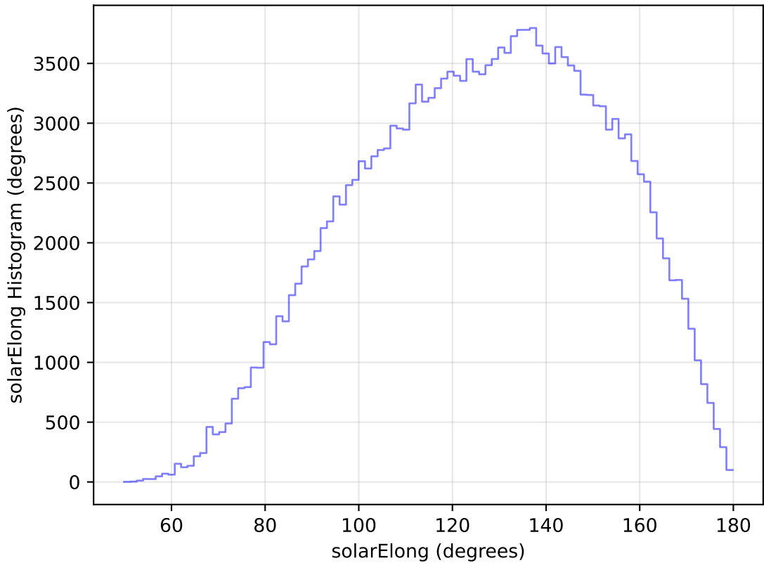
internal_u_expt30_nscale0.9v3.4_10yrs WFD g band: solarElong Histogram
