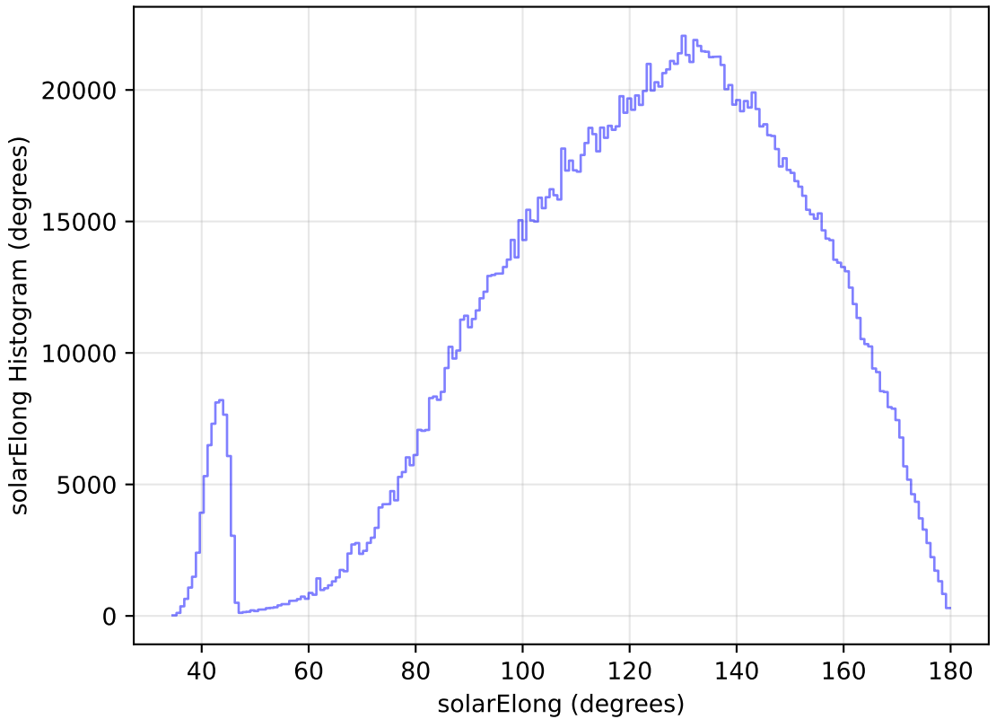
internal_u_expt30_nscale0.9v3.4_10yrs WFD all bands: solarElong Histogram
