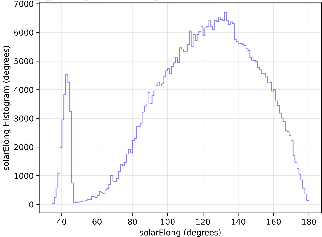
internal_u_expt30_nscale0.9v3.4_10yrs All sky z band: solarElong Histogram
