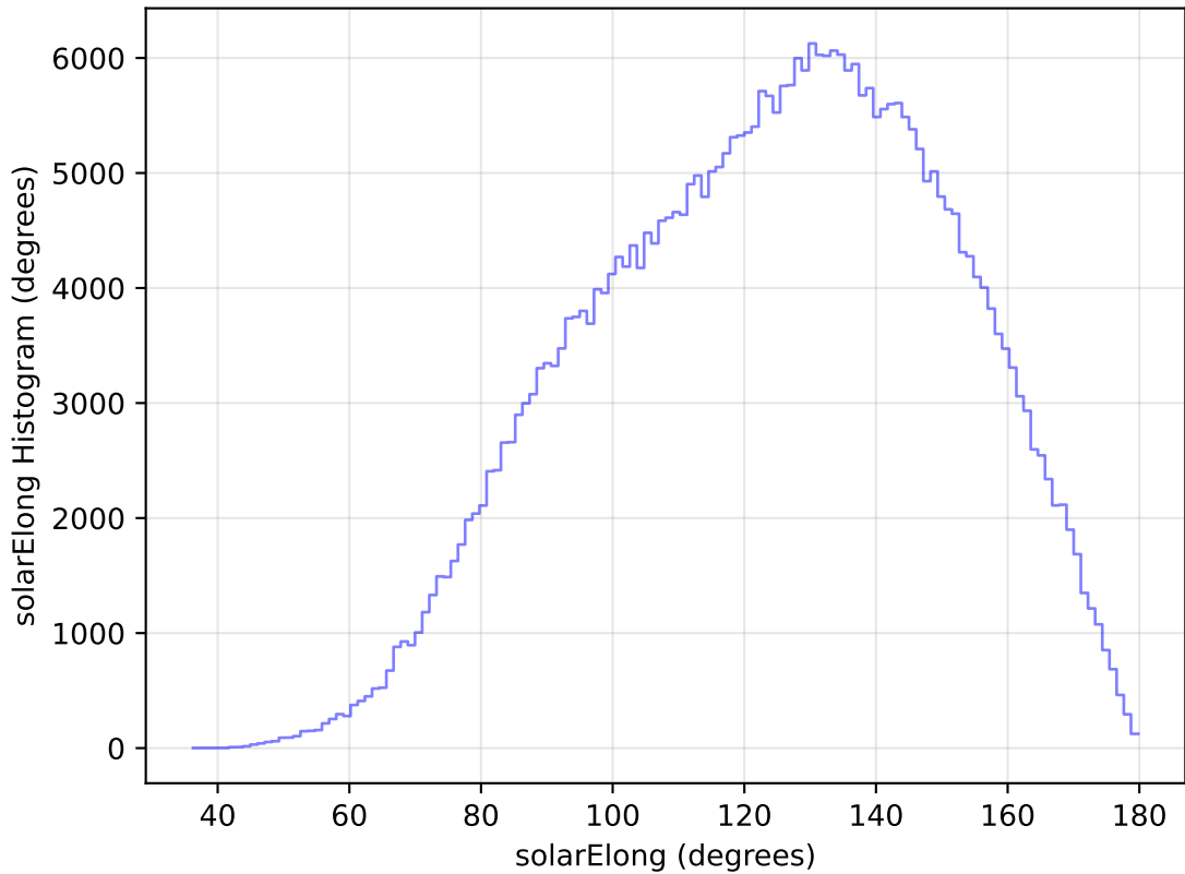
internal_u_expt30_nscale0.9v3.4_10yrs All sky y band: solarElong Histogram
