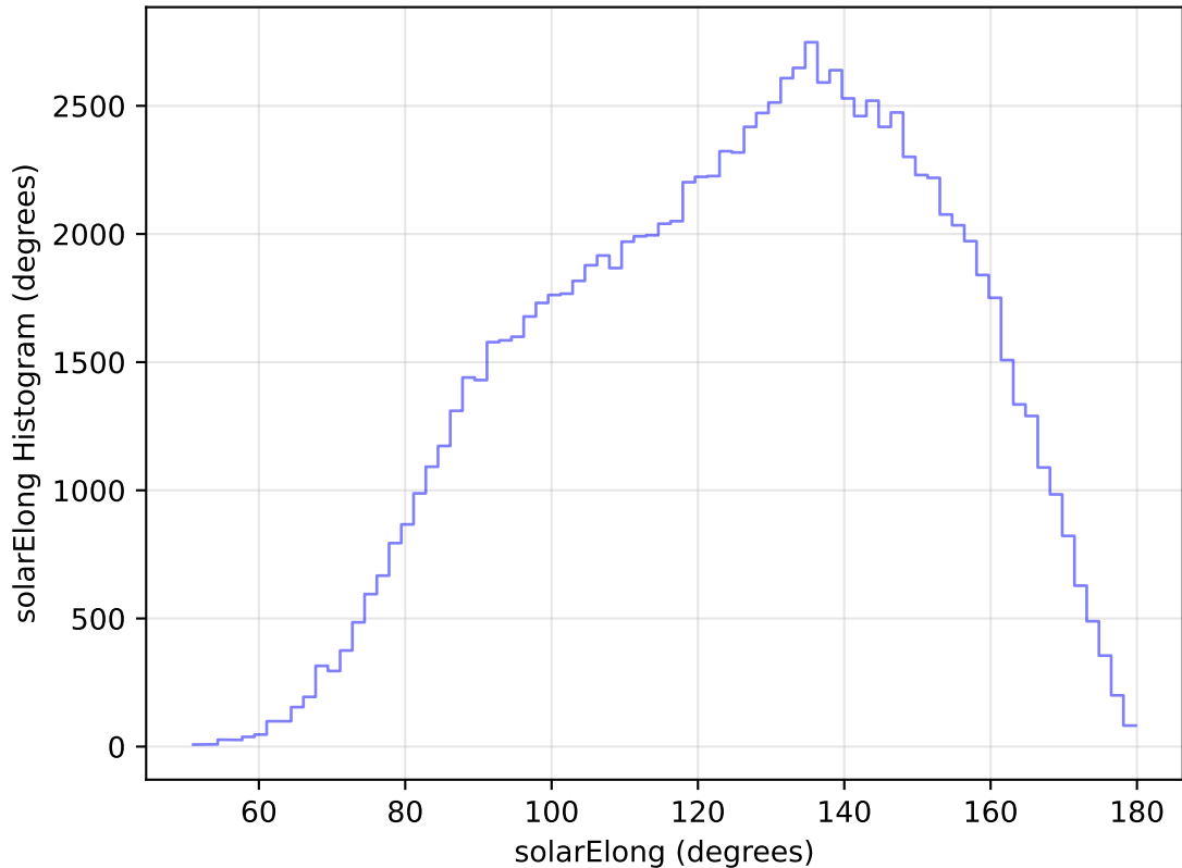
internal_u_expt30_nscale0.9v3.4_10yrs All sky u band: solarElong Histogram
