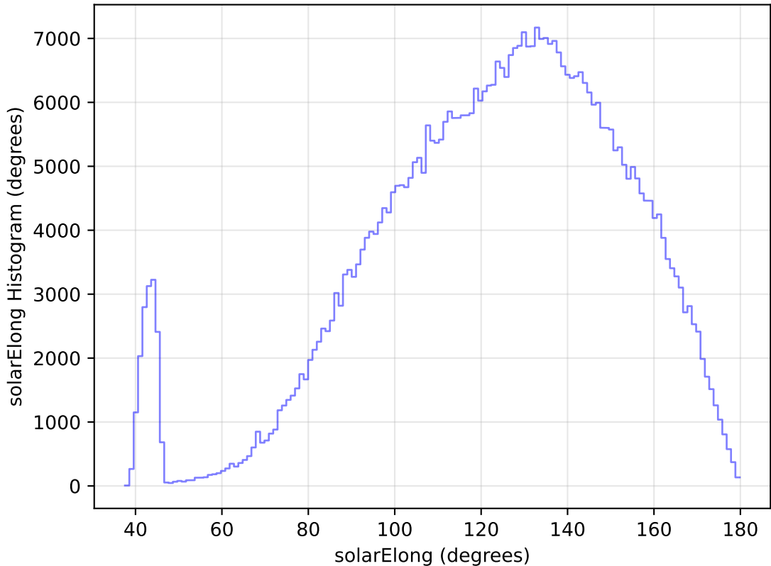
internal_u_expt30_nscale0.9v3.4_10yrs All sky r band: solarElong Histogram
