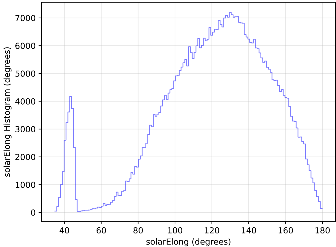
internal_u_expt30_nscale0.9v3.4_10yrs All sky i band: solarElong Histogram
