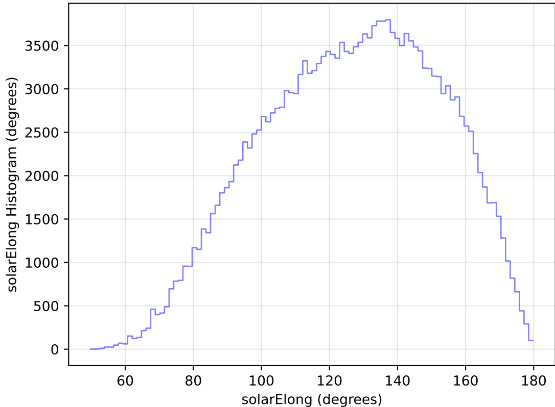
internal_u_expt30_nscale0.9v3.4_10yrs All sky g band: solarElong Histogram
