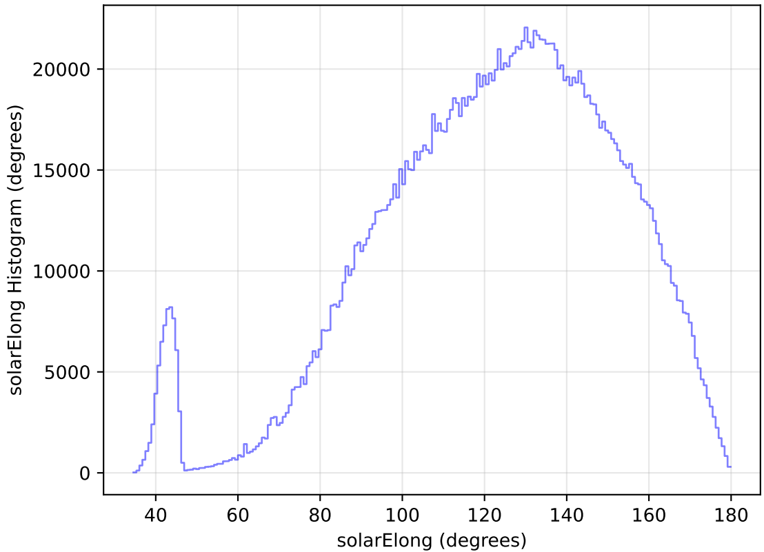
internal_u_expt30_nscale0.9v3.4_10yrs All sky all bands: solarElong Histogram
