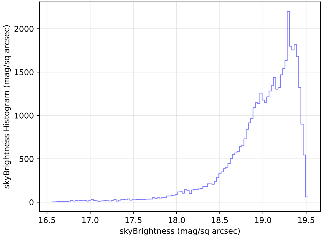
internal_u_expt30_nscale0.9v3.4_10yrs Yr 1 z band: skyBrightness Histogram
