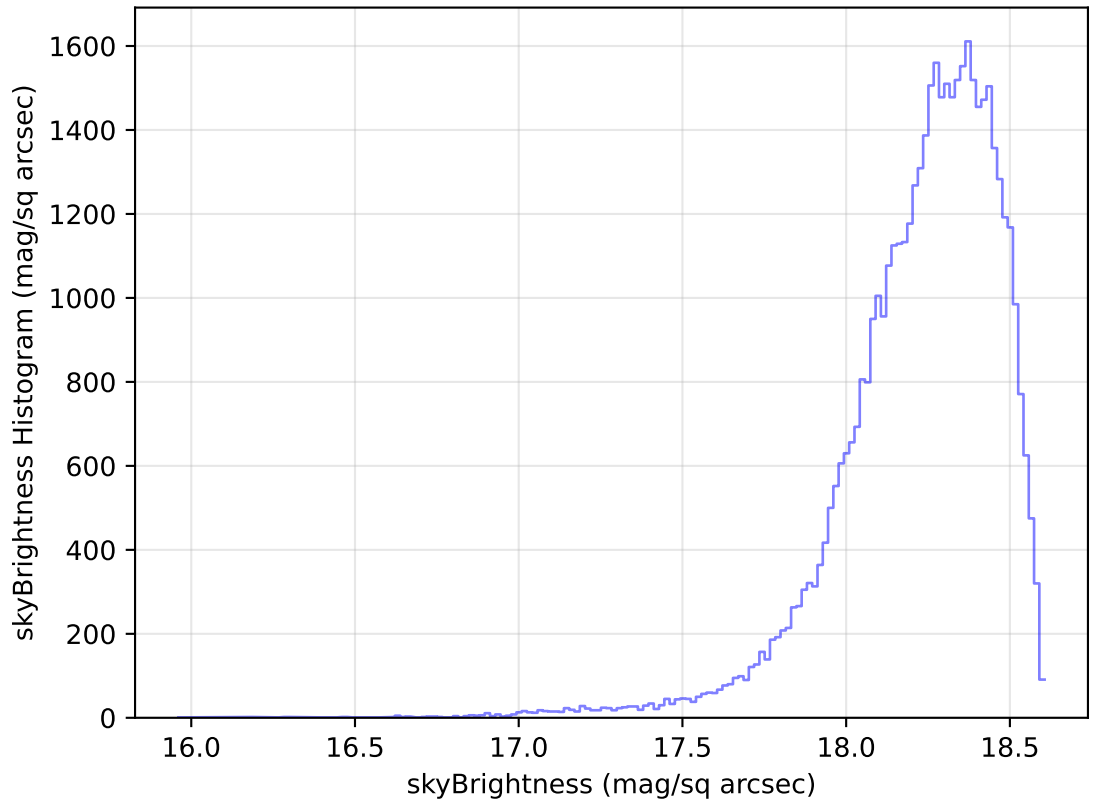
internal_u_expt30_nscale0.9v3.4_10yrs Yr 1 y band: skyBrightness Histogram
