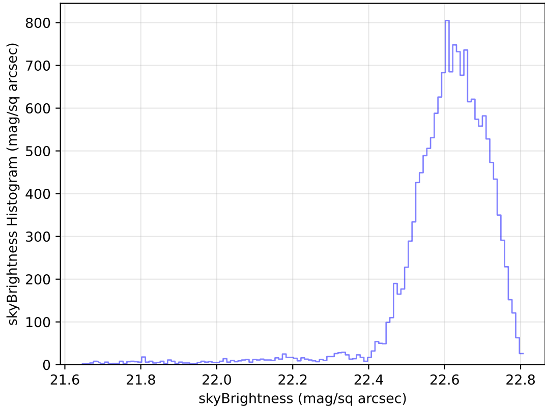
internal_u_expt30_nscale0.9v3.4_10yrs Yr 1 u band: skyBrightness Histogram
