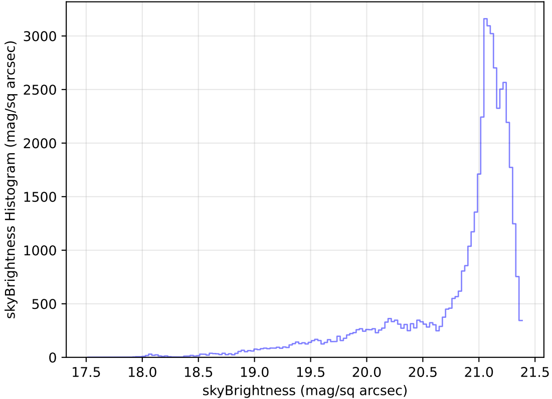
internal_u_expt30_nscale0.9v3.4_10yrs Yr 1 r band: skyBrightness Histogram
