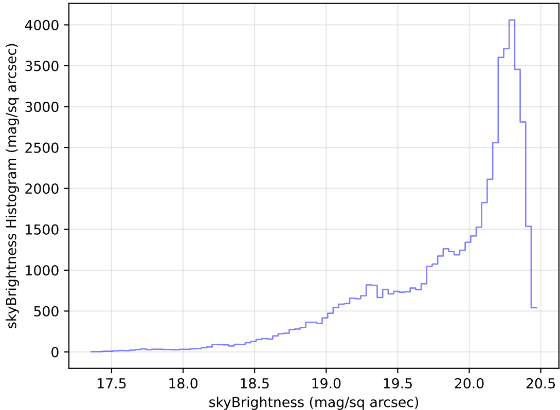
internal_u_expt30_nscale0.9v3.4_10yrs Yr 1 i band: skyBrightness Histogram
