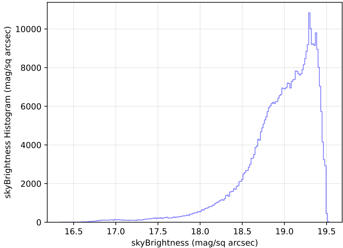
internal_u_expt30_nscale0.9v3.4_10yrs WFD z band: skyBrightness Histogram
