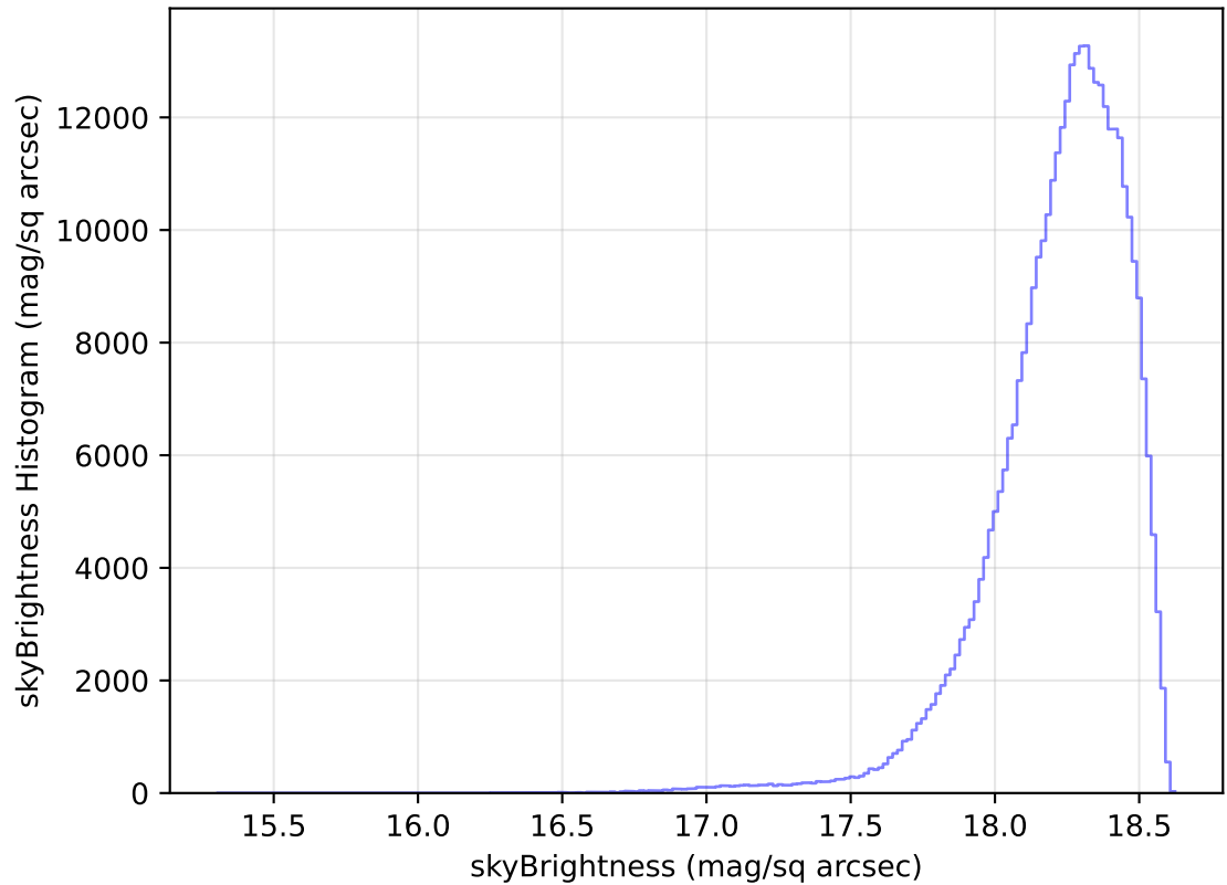
internal_u_expt30_nscale0.9v3.4_10yrs WFD y band: skyBrightness Histogram
