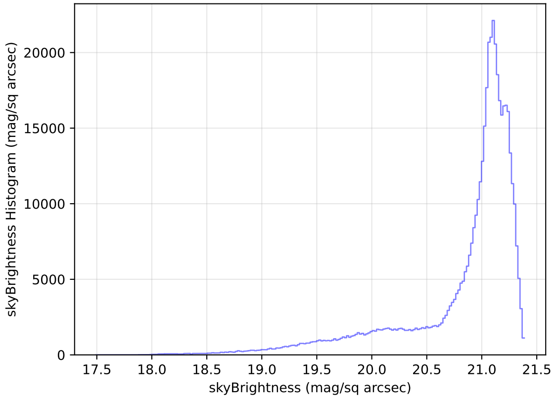
internal_u_expt30_nscale0.9v3.4_10yrs WFD r band: skyBrightness Histogram
