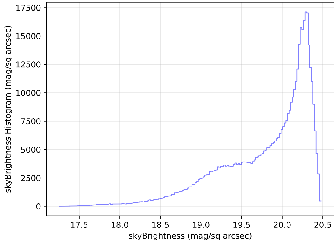
internal_u_expt30_nscale0.9v3.4_10yrs WFD i band: skyBrightness Histogram
