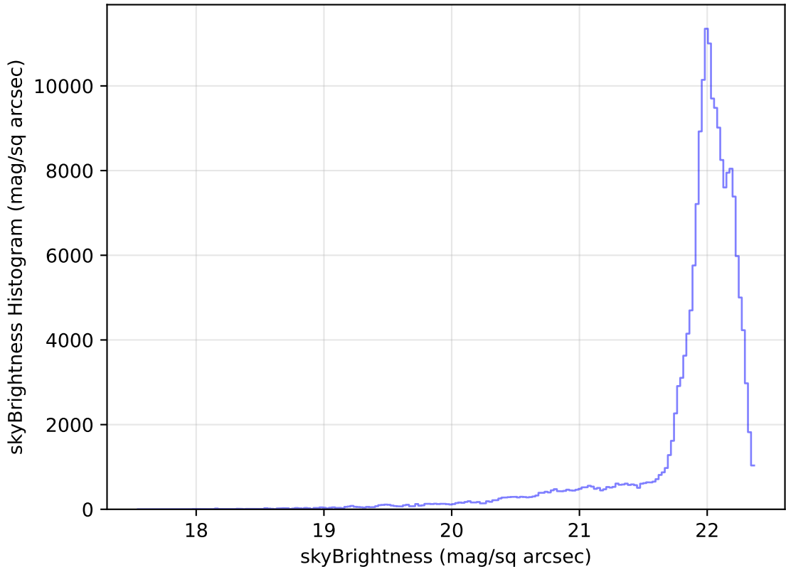
internal_u_expt30_nscale0.9v3.4_10yrs WFD g band: skyBrightness Histogram
