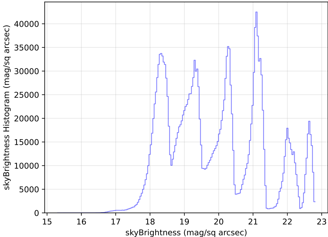
internal_u_expt30_nscale0.9v3.4_10yrs WFD all bands: skyBrightness Histogram
