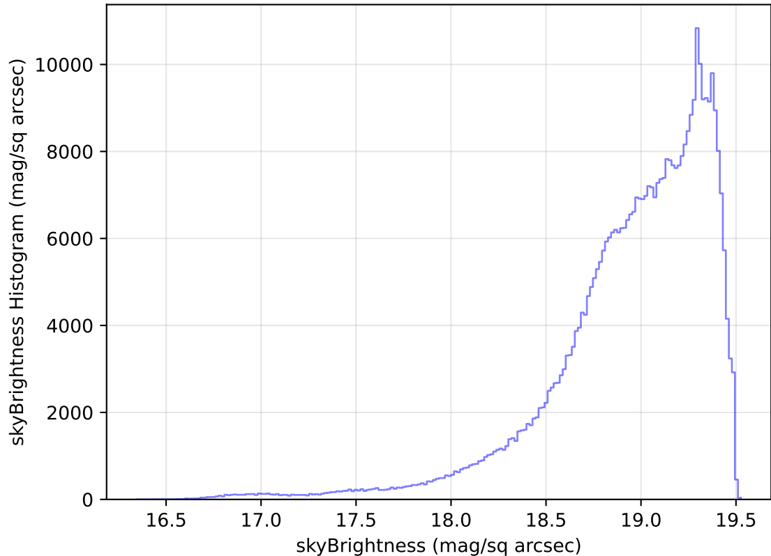
internal_u_expt30_nscale0.9v3.4_10yrs All sky z band: skyBrightness Histogram
