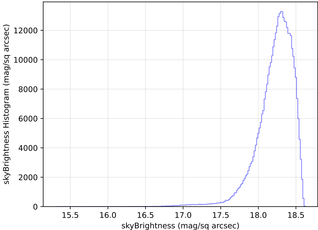
internal_u_expt30_nscale0.9v3.4_10yrs All sky y band: skyBrightness Histogram
