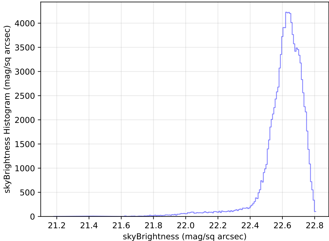
internal_u_expt30_nscale0.9v3.4_10yrs All sky u band: skyBrightness Histogram
